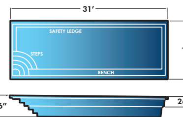
North Beach 12' x 31' x 4'6" Non-Diving Pool. Use of Diving Equipment is Prohibited
