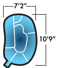
Kidney Spa with Spillover 7'2" x 10'9" x 37"
