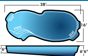
Dolphin I 16' x 38' x 6'6" Non-Diving Pool. Use of Diving Equipment is Prohibited
