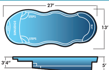
Funledge 13' x 27' x 5' Non-Diving Pool. Use of Diving Equipment is Prohibited
