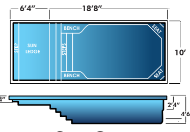
Sun Cove 10' x 25' x 4'6" Non-Diving Pool. Use of Diving Equipment is Prohibited
