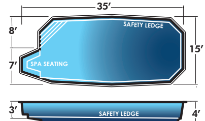
Honolulu I 15' x 35' x 4' Non-Diving Pool. Use of Diving Equipment is Prohibited
