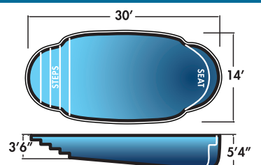
Waikiki 14' x 30' x 5'4" Non-Diving Pool. Use of Diving Equipment is Prohibited
