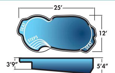
Cancun 12' x 25' x 5'4" Non-Diving Pool. Use of Diving Equipment is Prohibited
