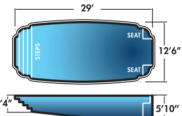
Acapulco 13' x 29' x 5'10" Non-Diving Pool. Use of Diving Equipment is Prohibited
