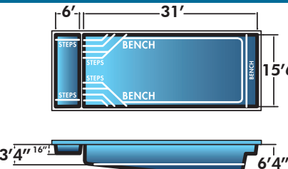
Island Beach 15'6" x 37' x 6'4" Non-Diving Pool. Use of Diving Equipment is Prohibited
