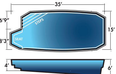
Honolulu II 15' x 35' x 6' Non-Diving Pool. Use of Diving Equipment is Prohibited
