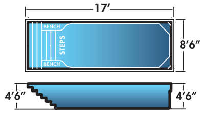
Eagle Ray 8'6" x 17' x 4'6" Non-Diving Pool. Use of Diving Equipment is Prohibited
