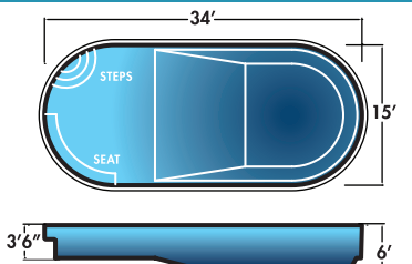
Costa Rica 15' x 34' x 6' Non-Diving Pool. Use of Diving Equipment is Prohibited
