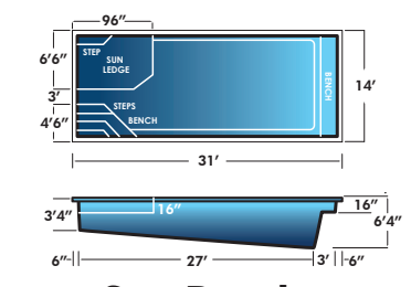
Sun Beach 14' x 31' x 6'4" Non-Diving Pool. Use of Diving Equipment is Prohibited
