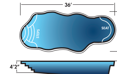
Oasis II 15'6" x 36' x 6'5" Non-Diving Pool. Use of Diving Equipment is Prohibited
