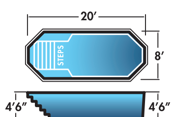
Sunfish 8' x 20' x 4'6" Non-Diving Pool. Use of Diving Equipment is Prohibited
