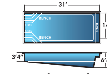
Palm Beach 14' x 31' x 6'4" Non-Diving Pool. Use of Diving Equipment is Prohibited
