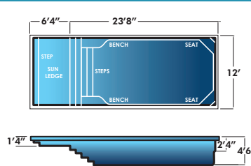
Beach Cove 12' x 30' x 4'6" Non-Diving Pool. Use of Diving Equipment is Prohibited
