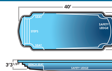
Orca Jr 16' x 40' x 6'3" Non-Diving Pool. Use of Diving Equipment is Prohibited
