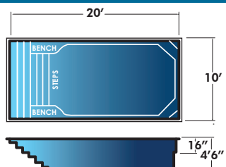
Key West 10' x 20' x 4'6" Non-Diving Pool. Use of Diving Equipment is Prohibited
