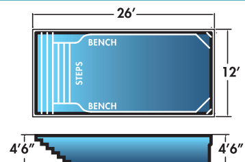
Stingray III 12' x 26' x 4'6" Non-Diving Pool. Use of Diving Equipment is Prohibited
