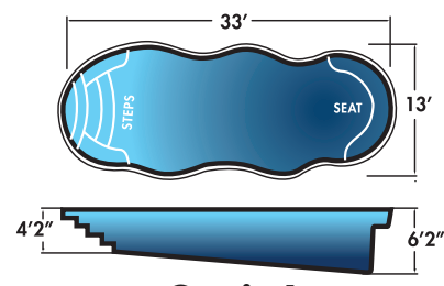
Oasis I 13' x 33' x 6'2" Non-Diving Pool. Use of Diving Equipment is Prohibited
