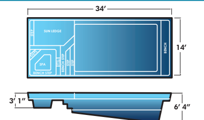
Spa Beach 14' x 34' x 6'4" Non-Diving Pool. Use of Diving Equipment is Prohibited
