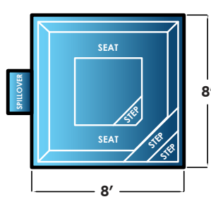
Square Spa with Spillover 8' x 8'
