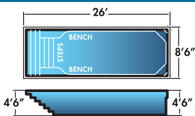
Stingray I 8'6" x 26' x 4'6" Non-Diving Pool. Use of Diving Equipment is Prohibited
