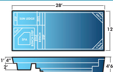
Spa Ray 12' x 28' x 4'6" Non-Diving Pool. Use of Diving Equipment is Prohibited
