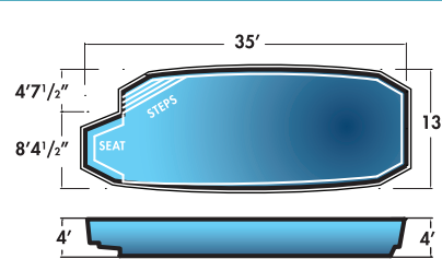
Azures I 13' x 35' x 4' Non-Diving Pool. Use of Diving Equipment is Prohibited
