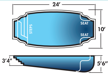
Bahamas 10' x 24' x 5'6" Non-Diving Pool. Use of Diving Equipment is Prohibited
