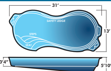
Tiger Shark 13' x 31' x 5'10" Non-Diving Pool. Use of Diving Equipment is Prohibited
