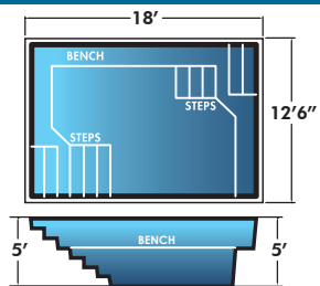
Aruba 12'6" x 18' x 5' Non-Diving Pool. Use of Diving Equipment is Prohibited
