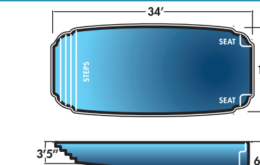
Maui 15' x 34' x 6'6" Non-Diving Pool. Use of Diving Equipment is Prohibited
