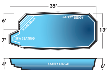
Azures II 13' x 35' x 6' Non-Diving Pool. Use of Diving Equipment is Prohibited
