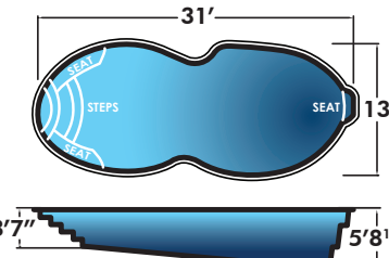
Angelfish 13' x 31' x 5'8" Non-Diving Pool. Use of Diving Equipment is Prohibited
